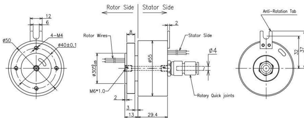
Rotary quick joints
